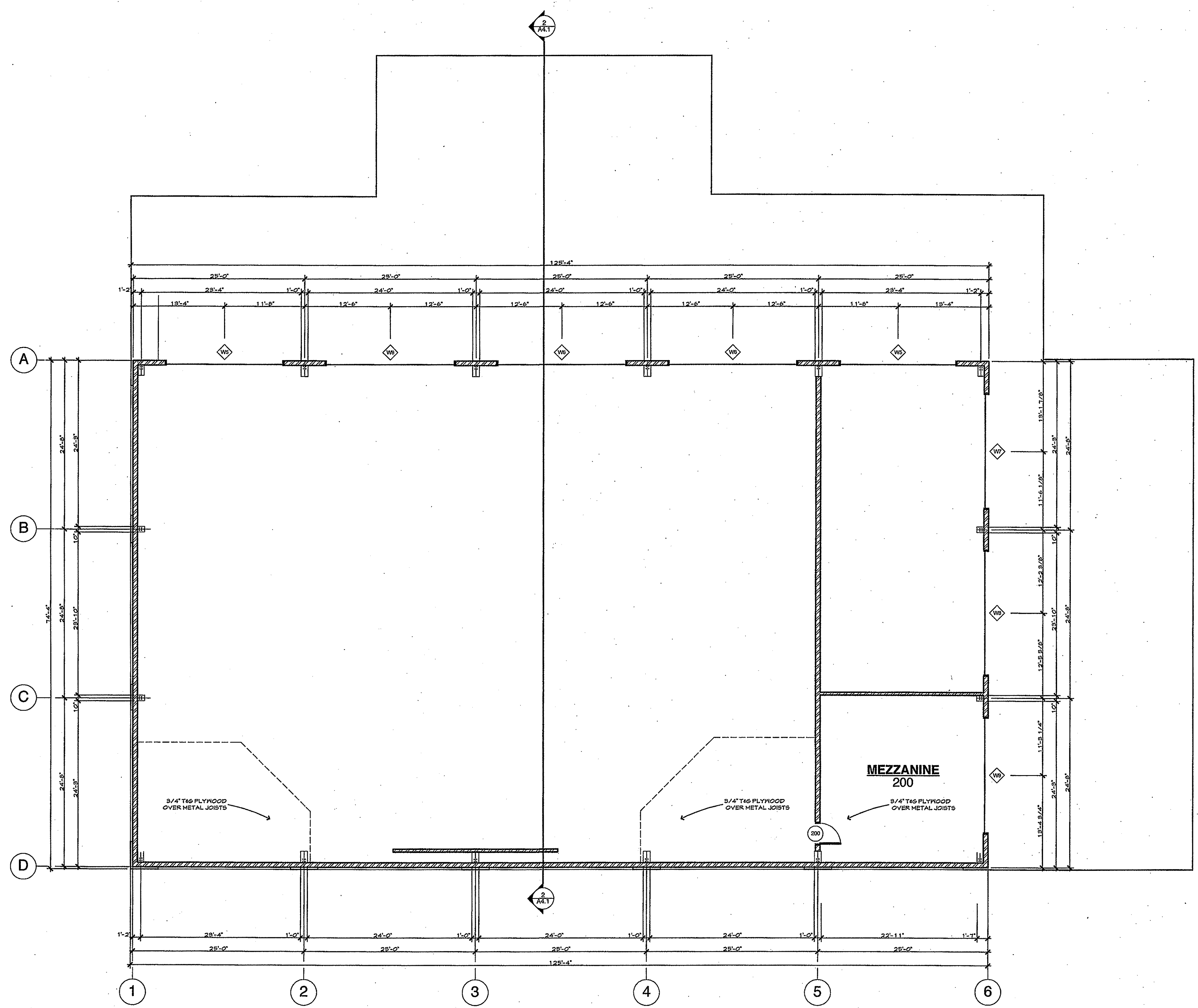
1 A2.1 Mezzanine Plan Scale 1/8" = 1'-0"
