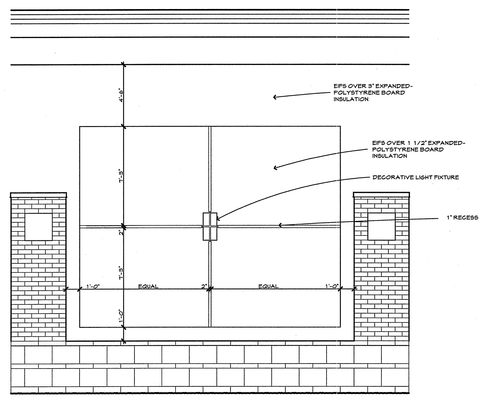
1 Enlarged Elevation A3.2 Scale 1/4" = 1' - 0"
