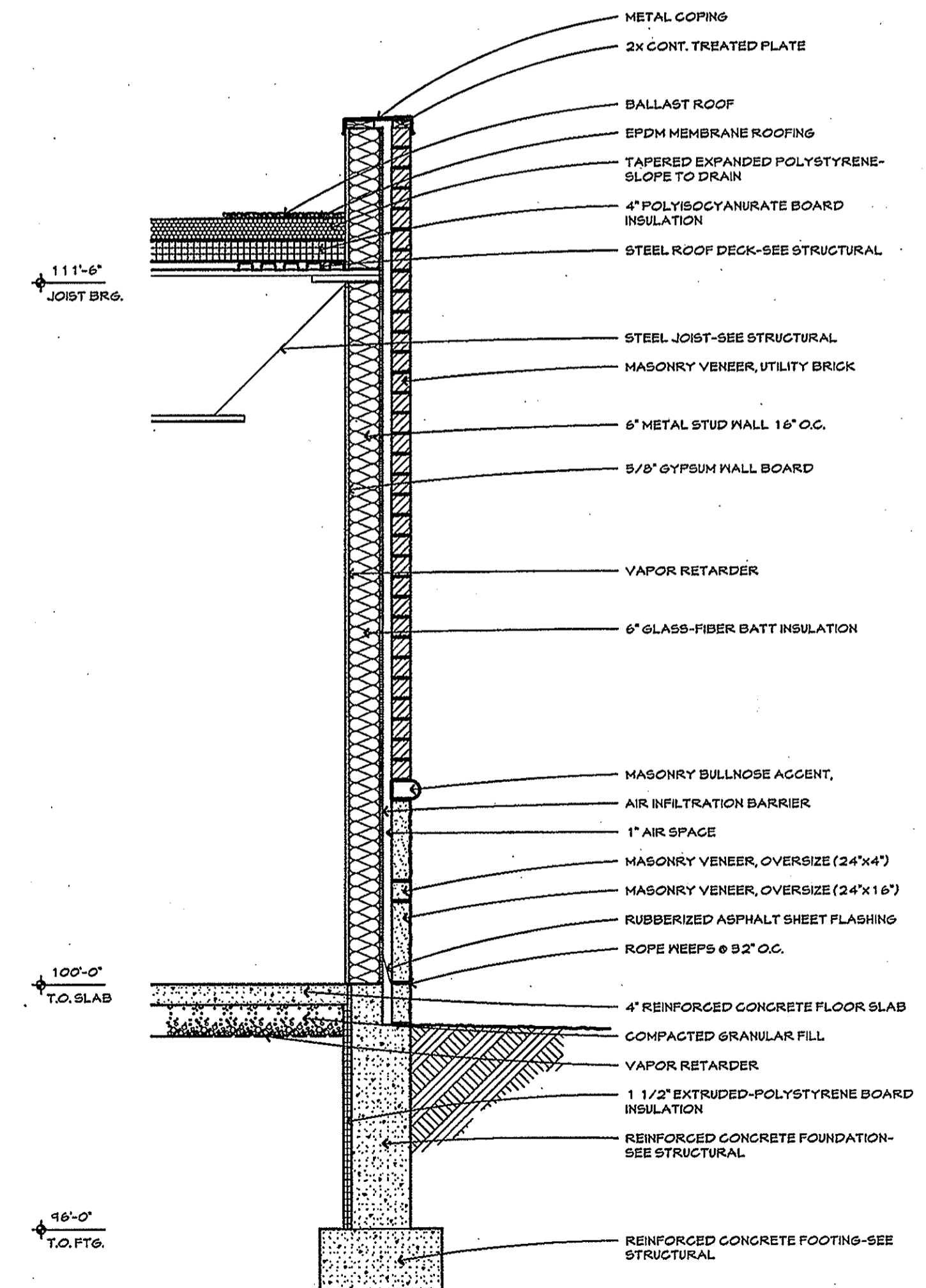
4 Wall Section A4.3 Scale 1/2" = 1'-0"
