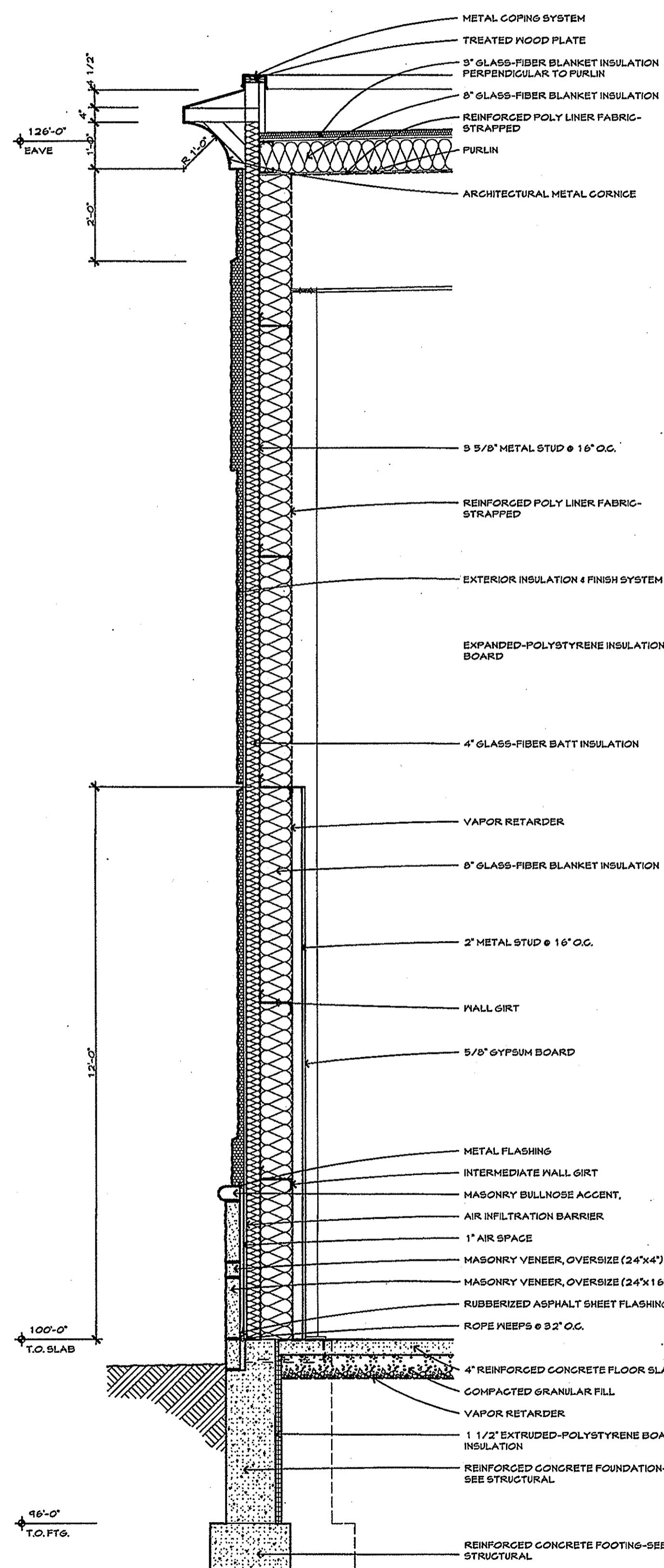
1 Wall Section A4.3 Scale 1/2" = 1'-0"
