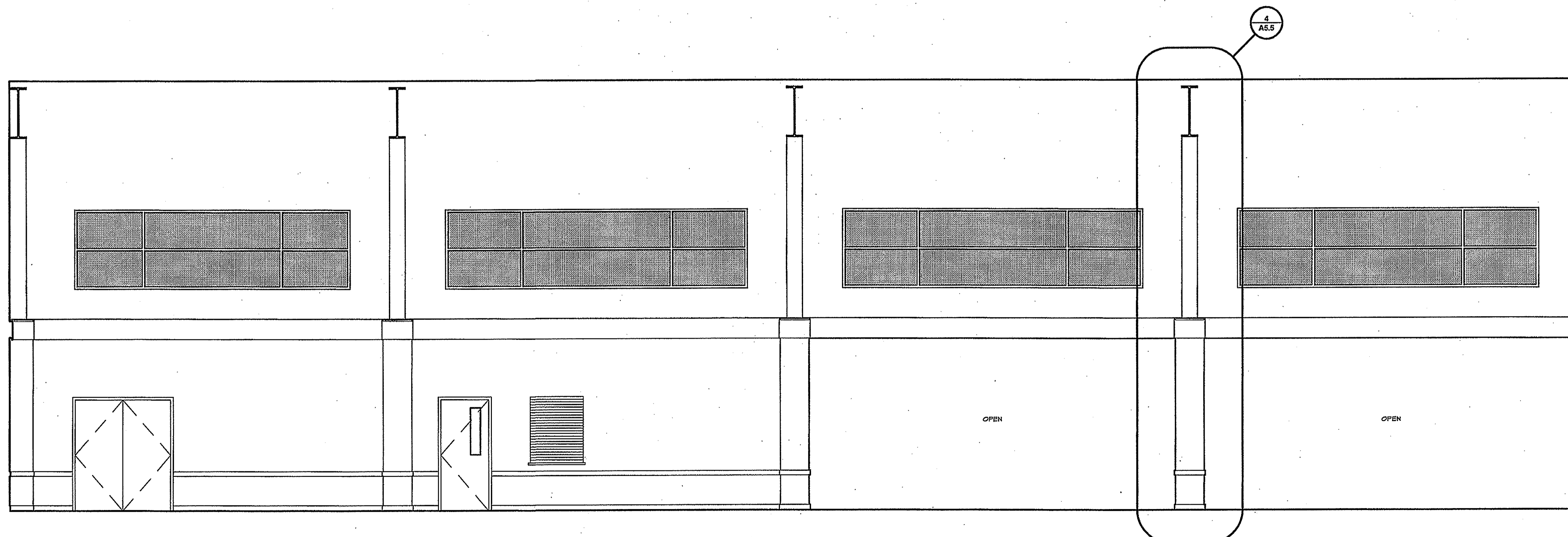
2 A5.4 Interior Elevation Scale 1/4" = 1'-0"
