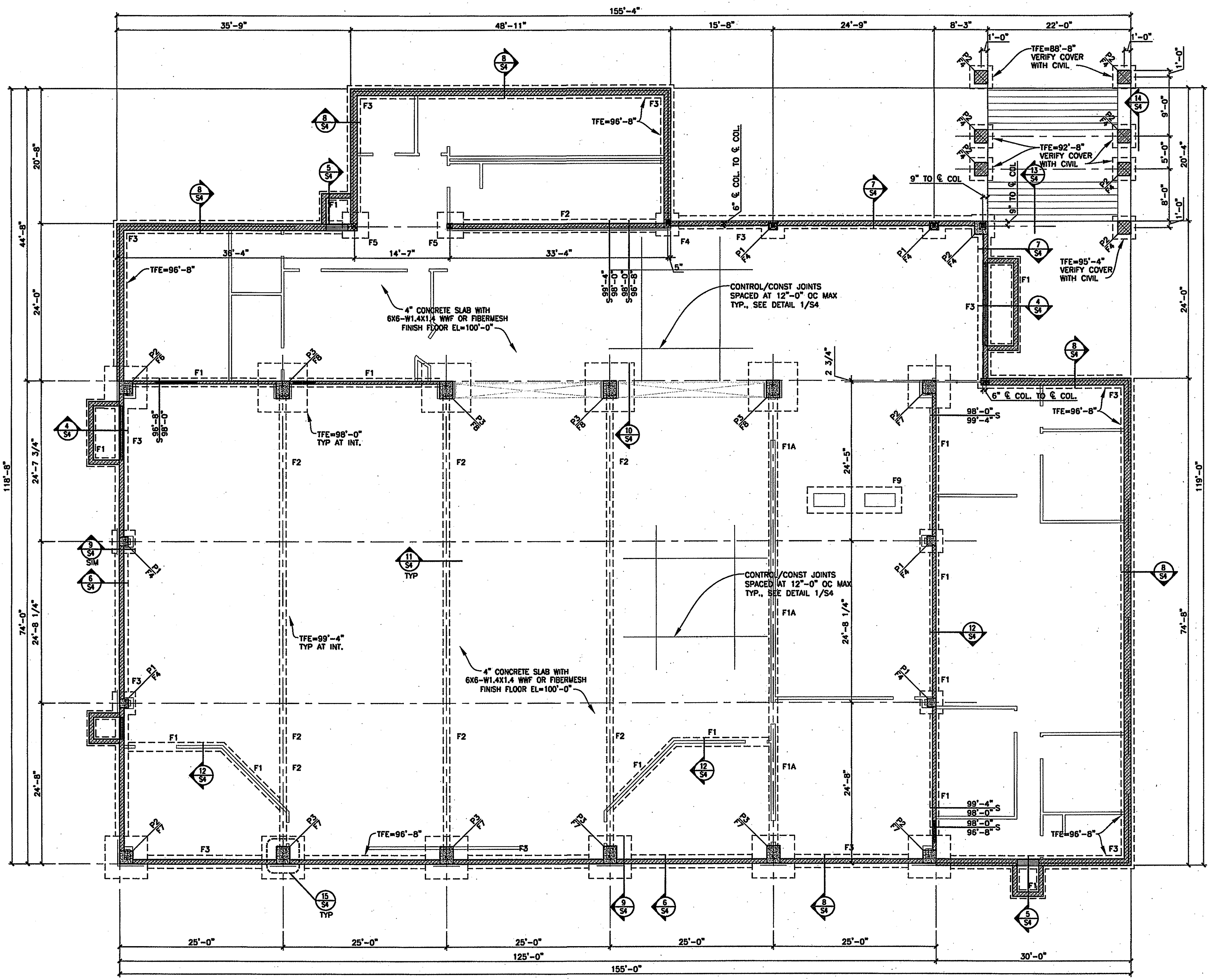
FOUNDATION PLAN 1/8"=1'-0" PLAN
